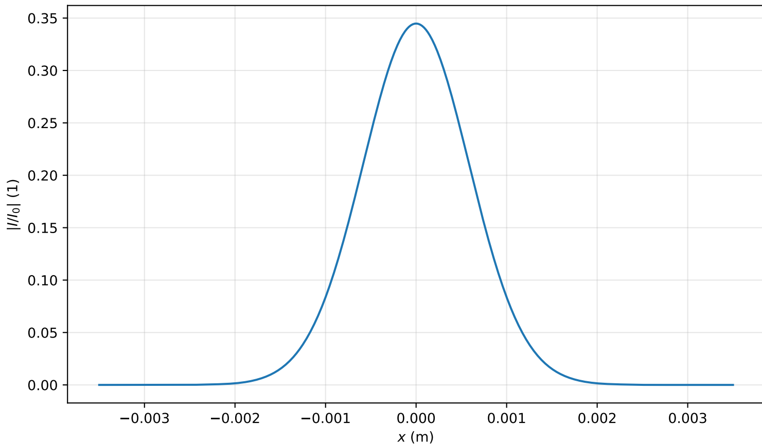
Intensity profile I(x, y = 0, z = 2.946m)/I_0 , P_{in}=0.1P_{cr} , artificial time
